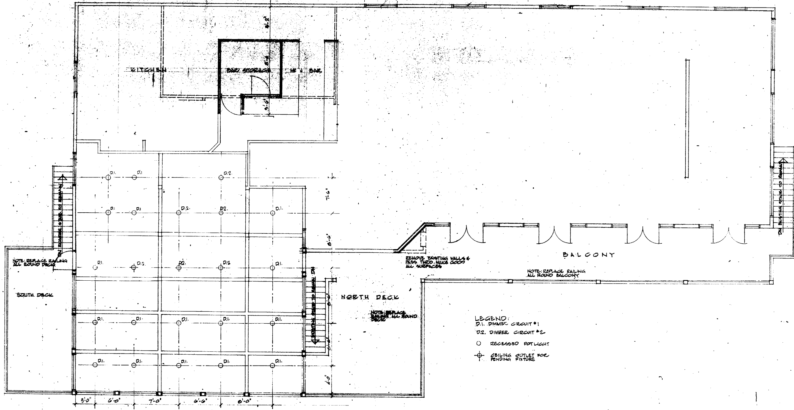
REFLECTED CEILING PLAN IN DINING ROOM SHOWING FALSE BEAMS SCALE: 1/4" = 1'-0"
