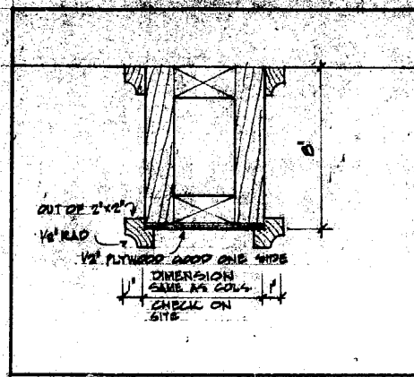
SECTION THRO FALSE BEAM SCALE: 3/4" = 1'-0"
