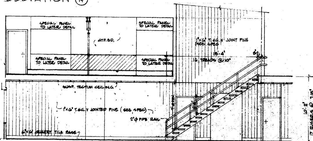
ELEVATIONAL SECTION & SECTION THRO STAIR
