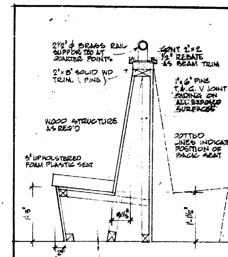
SECTION THRO FIXED SEATING IN DINING RM.
